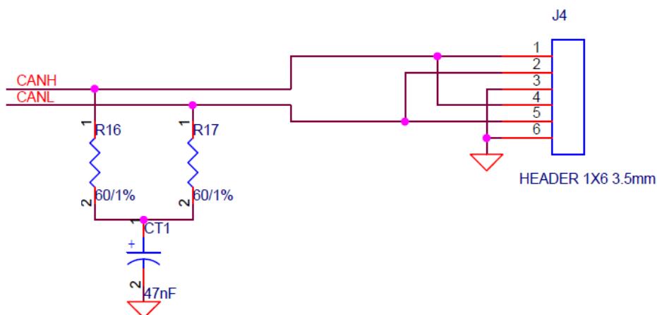
CAN bus schematic
