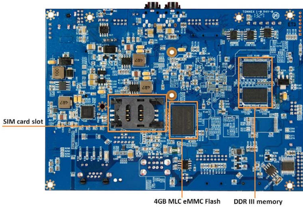
SBC2100 PCB Bottom View
