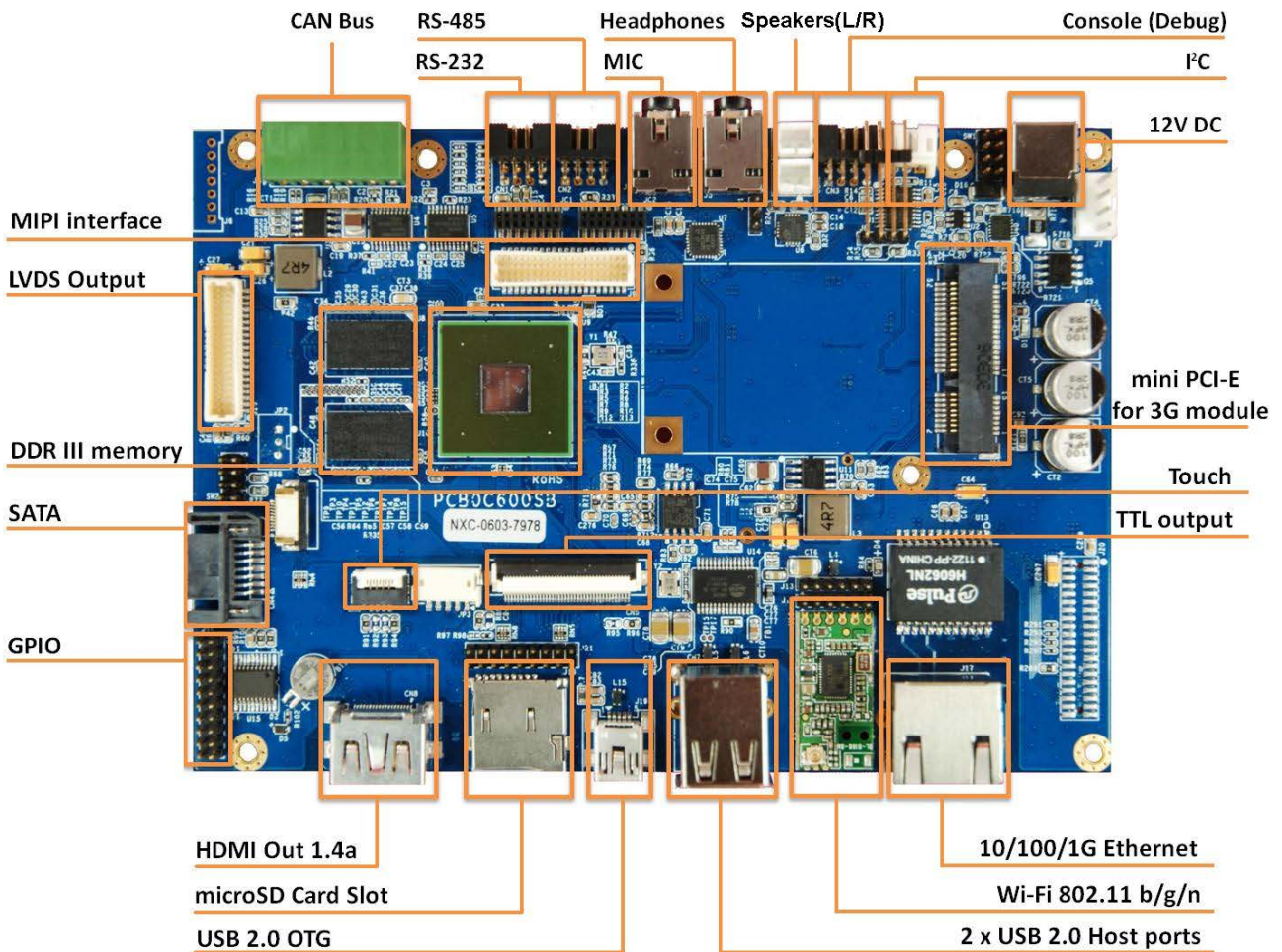
SBC2100 PCB Top View
